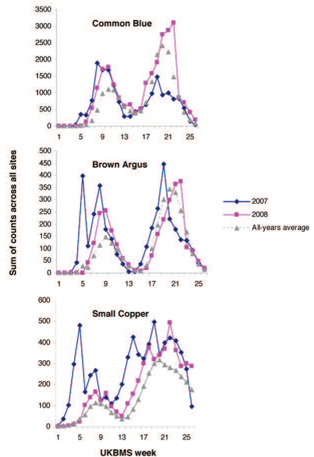
Figure 5. Flight times of Common Blue, Brown Argus and Small Copper counted on UKBMS transects. Note week 1= 1-7 April, week 26 = 23-29 September
