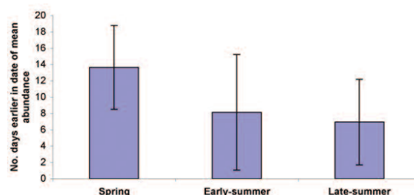
Figure 22. Mean ( \pm 1 s.d.) advance in mean flight date for species grouped by the time of year they fly
