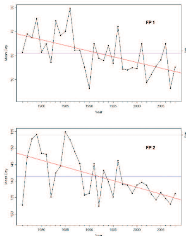
Figure 21. The date at which the mean flight date was recorded for the first flight period (FP1) and second flight period (FP2) of the Wall Brown since 1976. The blue line represents the average over the thirty-three year period, whilst the red line represents the trend (change in mean flight date over time) calculated from a linear regression
